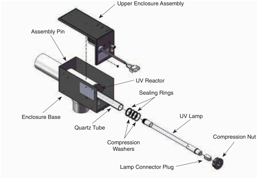
Figure 2: Mast3rPur System Exploded View
